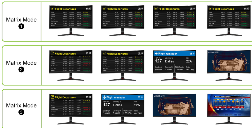
Matrix
